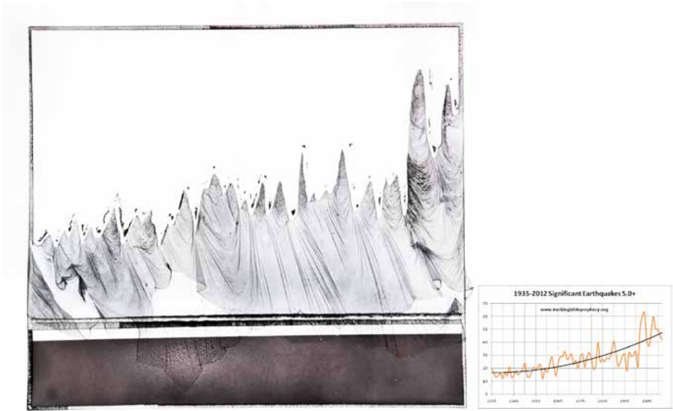
1935-2012 Significant Earthquakes Over 5.0
